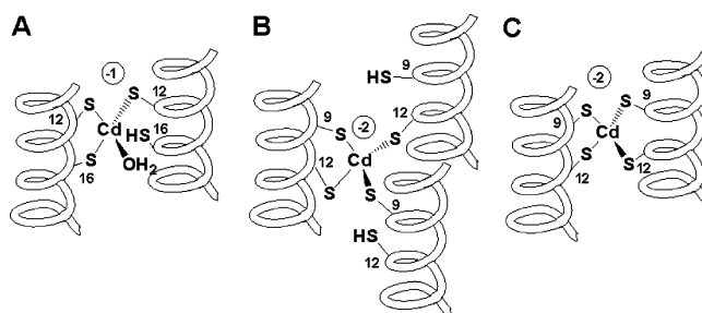
Scheme 2. Schematic Representation of Cd(II) Complexes of TRIL12CL16C (A) and TRIL9CL12C (B,C)
