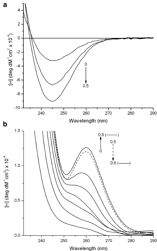
Figure 4. Circular dichroism difference spectra of pH titrations of Cd(II) into the solutions of 90 \mu\text{M} TRIL12CL16C in 50 mM TRIS buffer pH 8.5 (a) and 90 \mu\text{M} TRIL9CL12C in 50 mM TRIS buffer pH 8.5 (b).
