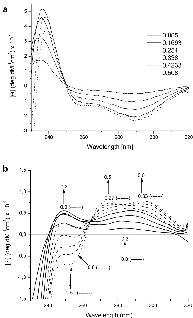
Figure 5. Circular dichroism difference spectra of titrations of Hg(II) into the solution of 50 mM CHES buffer pH 9.4 containing 90 \mu\text{M} TRIL12CL16C (a) and 90 \mu\text{M} TRIL9CL12C (b).
