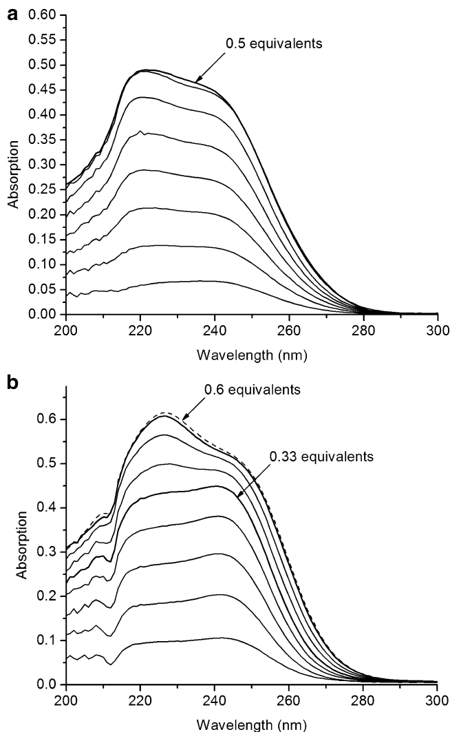
Figure 1. Difference spectra of titrations of Cd(II) into the solution of 50 mM TRIS buffer pH 8.5 containing 60 \mu\text{M} TRIL12CL16C (a) and 60 \mu\text{M} TRIL9CL12C (b).
