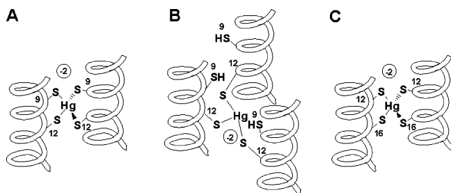
Scheme 3. Schematic Representation of Hg(II) Complexes of TRIL9CL12C (A,B) and TRIL12CL16C (C)
