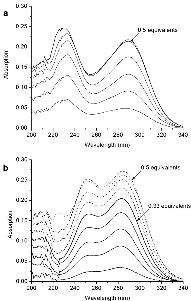
Figure 2. Difference spectra of titrations of Hg(II) into the solution of 50 mM CHES buffer pH 9.4 containing 60 \mu M TRIL12CL16C (a) and 60 \mu M TRIL9CL12C (b).
