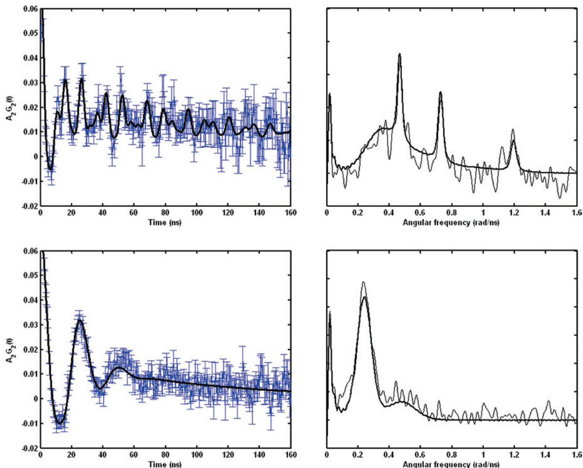
Figure 8. ^{111m}\text{Cd} PAC data for the Cd(II) complexes of TRIL12CL16C (upper) and TRIL9CL12C (lower) at pH 8.5. The experimental perturbation function and the fit (full line) and the Fourier transform of the experimental data (thin line) and of the fit (thick line) are shown on the left and the right, respectively.
