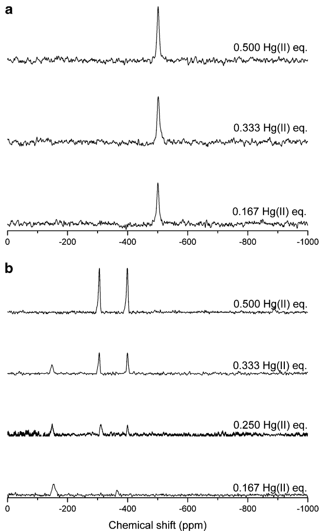
Figure 7. ^{199}\text{Hg} NMR spectra of subsequent titrations of ^{113}\text{Hg}(\text{II}) into the solution containing 10 mM TRIL12CL16C (a) and 10 mM TRIL9CL12C (b) at pH 9.4.
