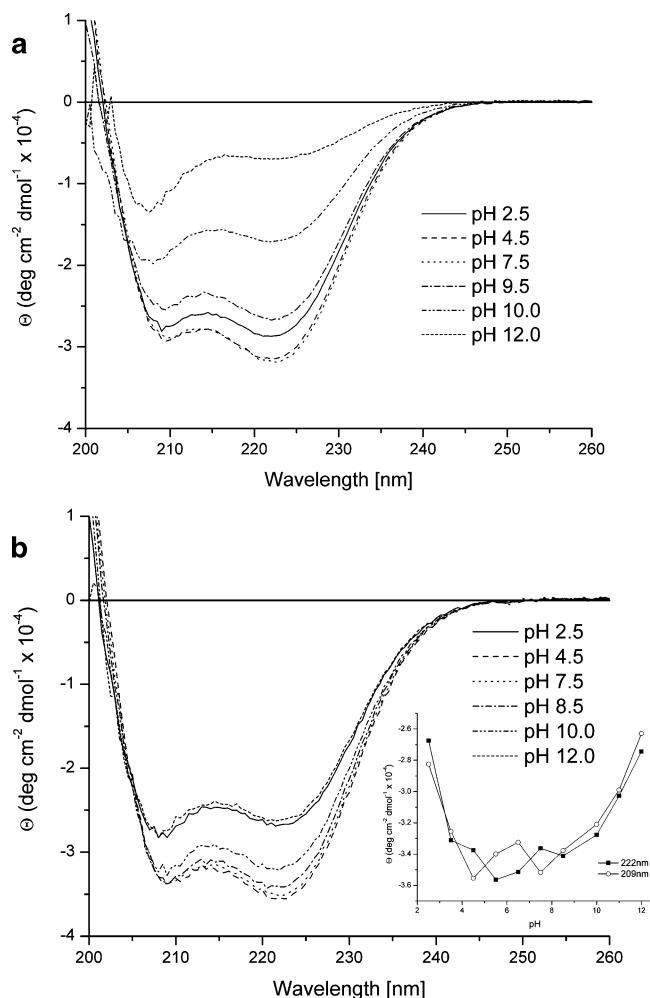
Figure 3. Far-UV circular dichroism spectra of pH titrations of TRIL12CL16C (a) and TRIL9CL12C (b). Changes in ellipticity at 209 and 222 nm are plotted as a function of pH in the inset.
