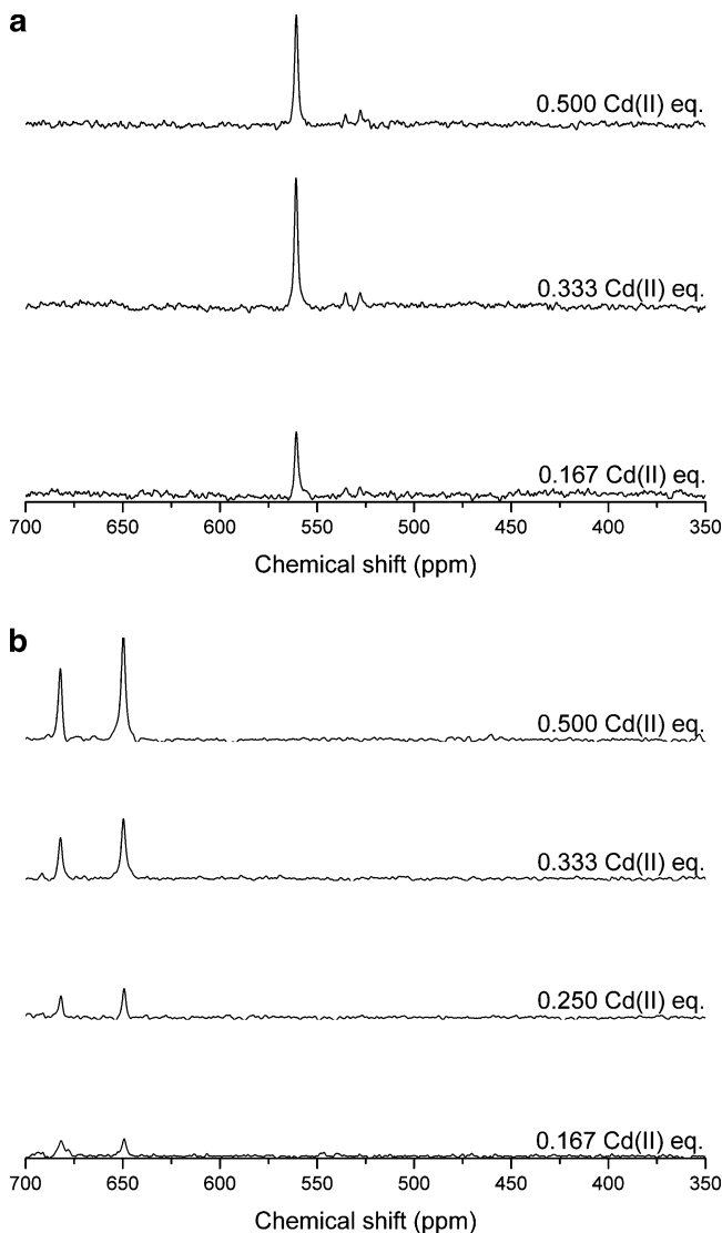
Figure 6. ^{113}\text{Cd} NMR spectra of subsequent titrations of ^{113}\text{Cd}(\text{II}) into the solution containing 10 mM TRIL12CL16C (a) and 10 mM TRIL9CL12C (b) at pH 8.5.
